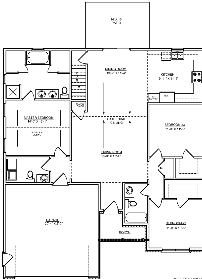
1ST FLOOR LAYOUT SCALE: 1/4" = 1'-0"
