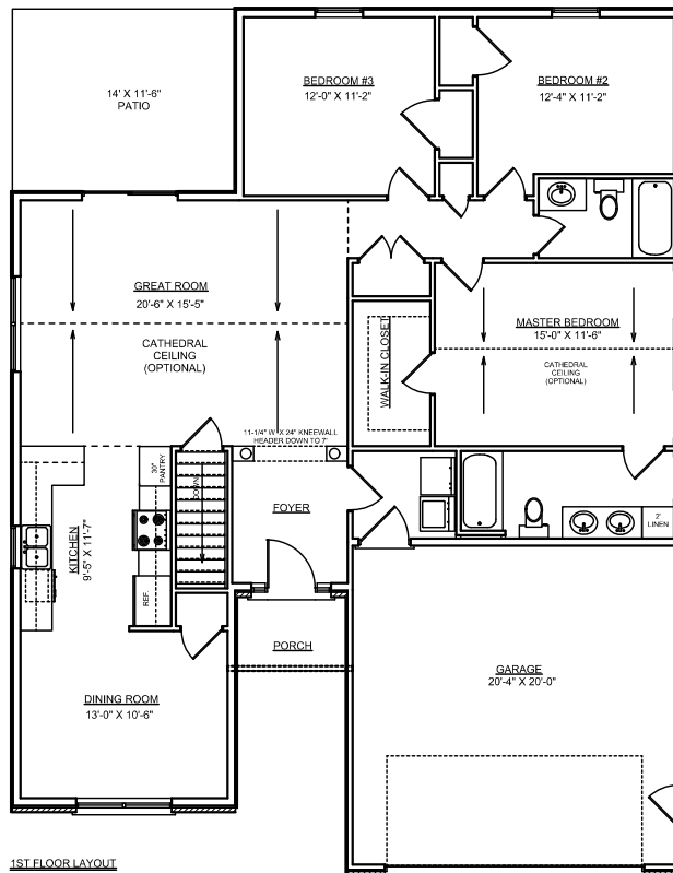
1ST FLOOR LAYOUT
