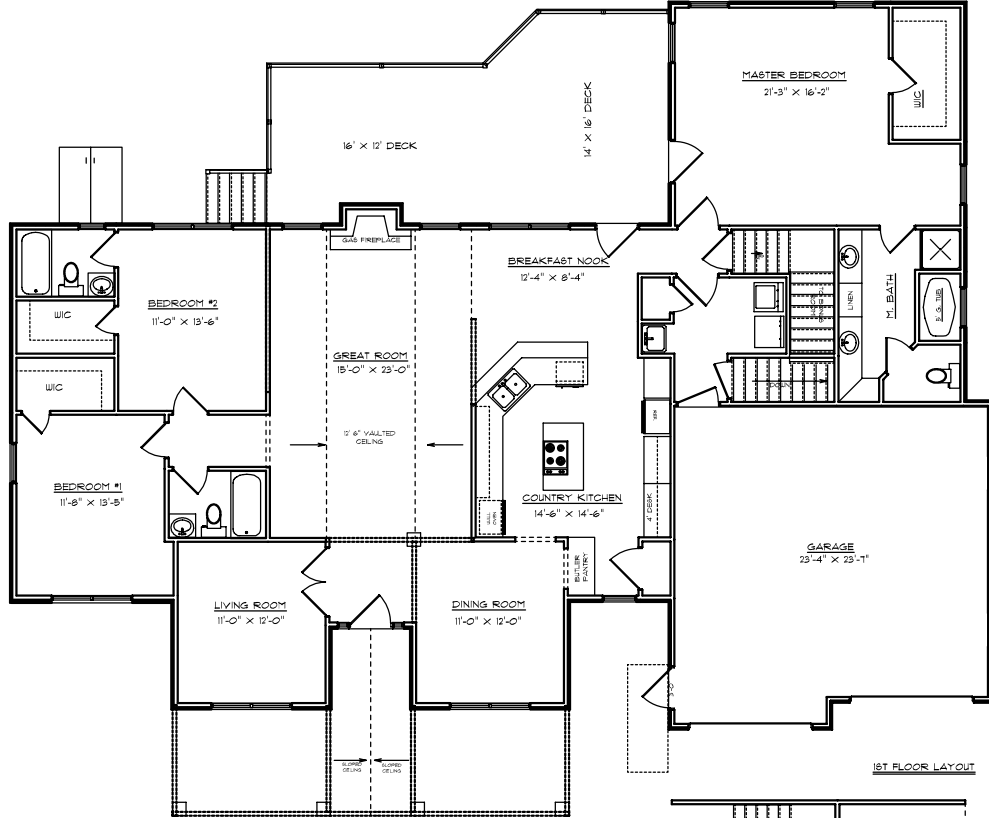
ARCHITECTURAL DETAILS OPTIONAL
